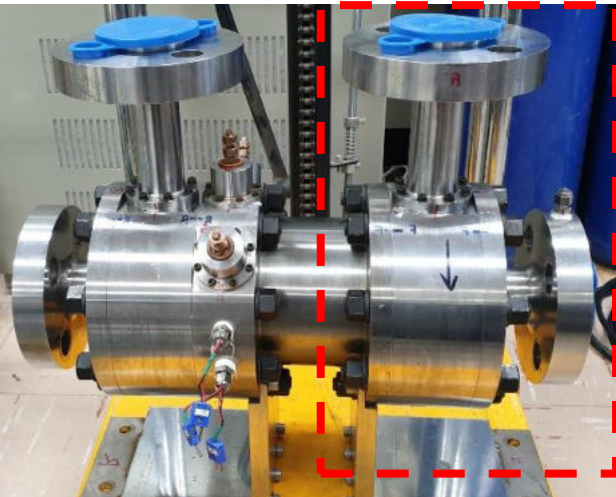
Turbo-Alternator-compressor (TAC)
