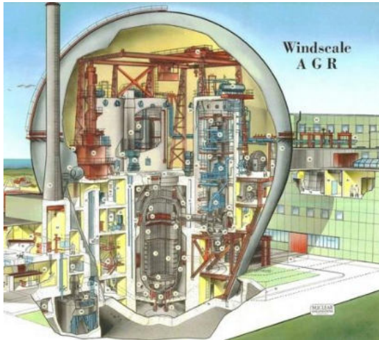
1965 – AGR, theengineer.co.uk
