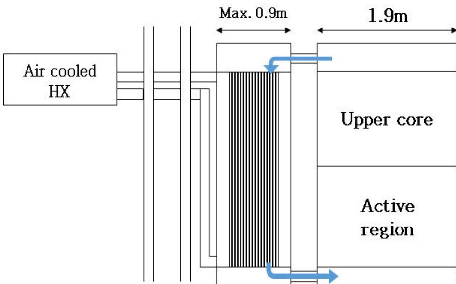
<PDHR schematic diagram>
