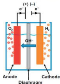
Alkaline electrolyzer
