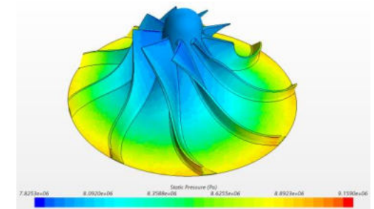
RANS simulation results (STAR-CCM+)
