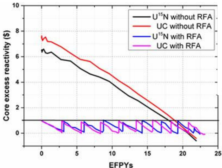
<Excess reactivity of MMR core>
