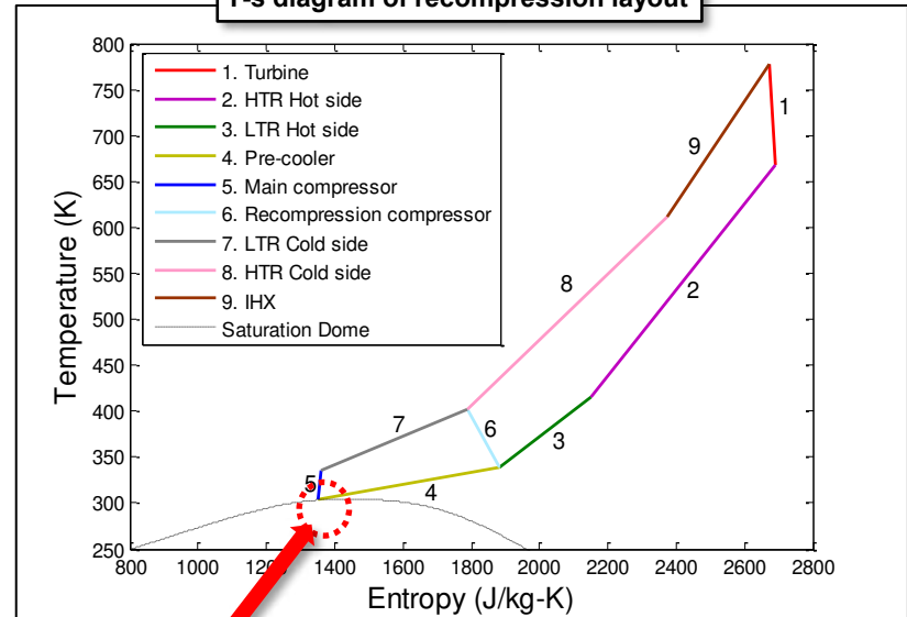
T-s diagram of recompression layout
