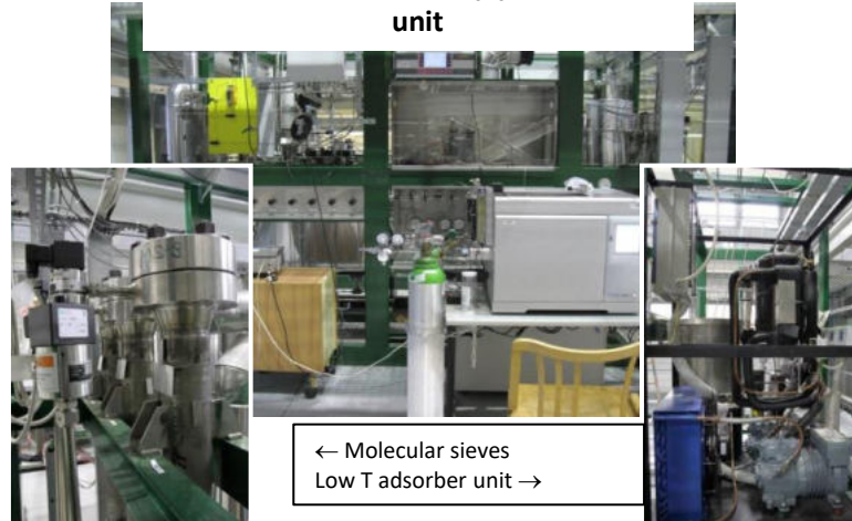
View of the HTHL1 loop purification unit
