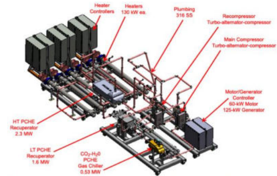
Engineering drawing of the piping layout for the S-CO 2 recompression Brayton Cycle.
