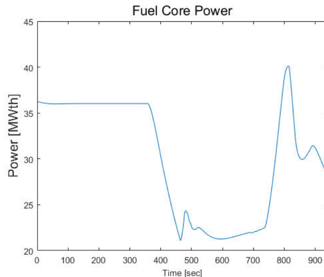
<Reactor power of MMR in marine propulsion>
