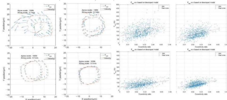
Fig. Lubrication analysis for each test
