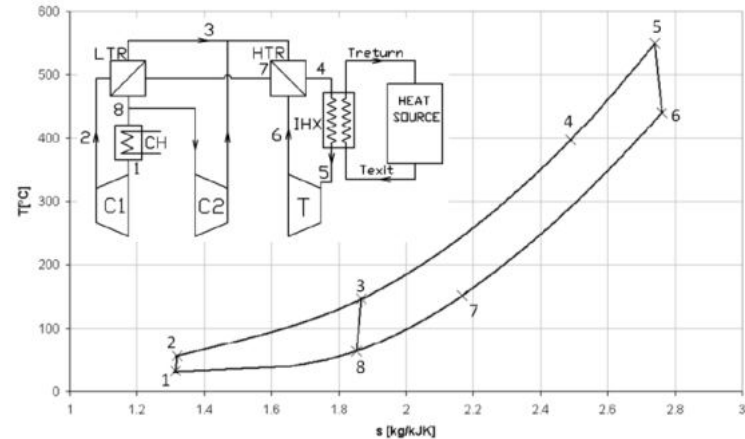
Recompression Cycle Temperature - Entropy Diagram
