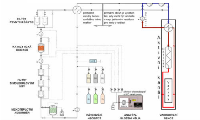
Scheme of the HTHL1 loop
