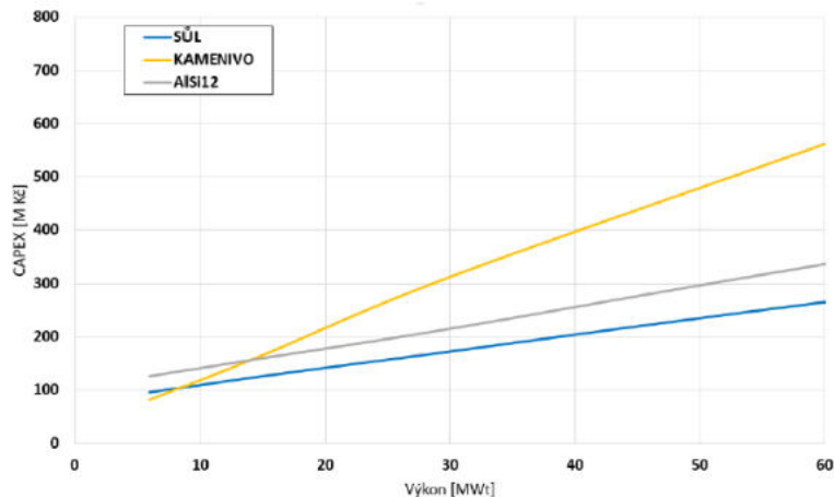
CAPEX for Constant capacity (150 MWht) and variable power
