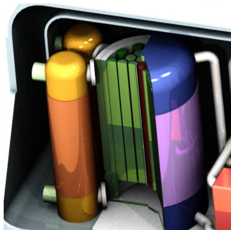
<Configuration of PDHR>
