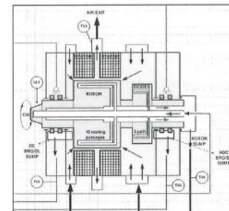
Figure 1: ALPS HS-Generator lubrication and cooling schematic.
