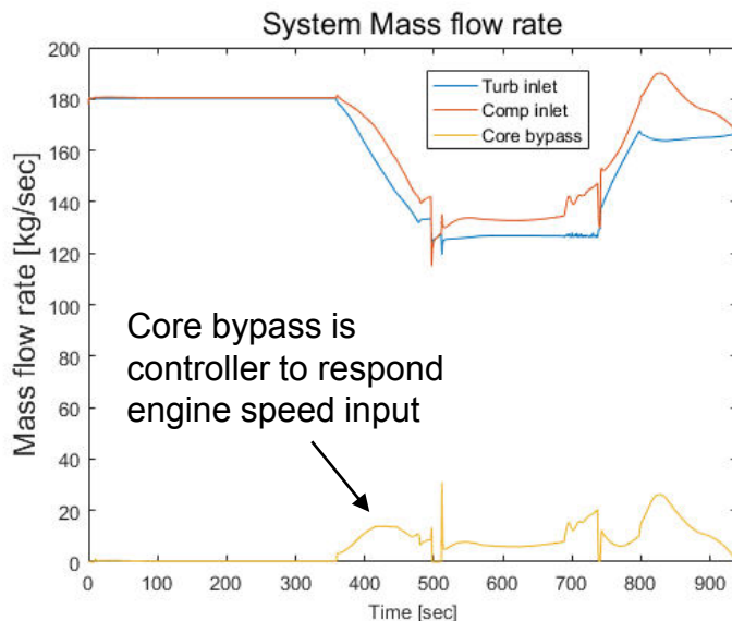
<System and bypass mass flow rate of MMR in marine propulsion>
