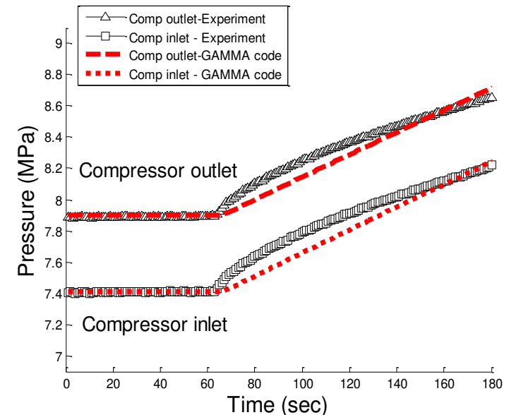
<SCO 2 PE facility modeling with modified GAMMA+ code>
