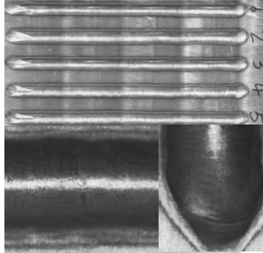
Laser-wire (LW) DED
