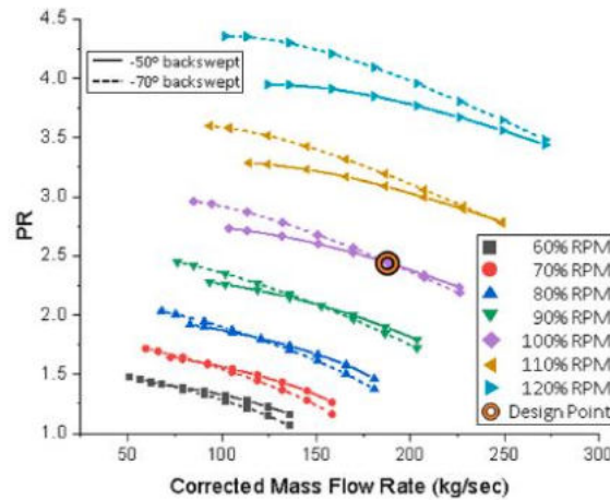
Compressor Map
