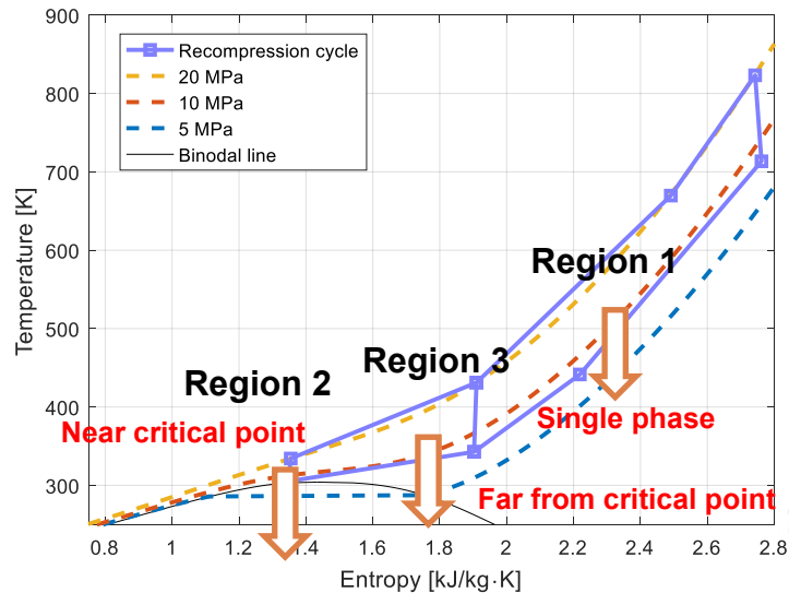
Fig. T-S diagram for CO 2 with depressurization
