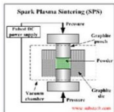
Sintering via SPS Pressure: 40 / 50 MPa Time: 10 min Temperature: 950 degree C
