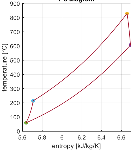
T-s diagram
