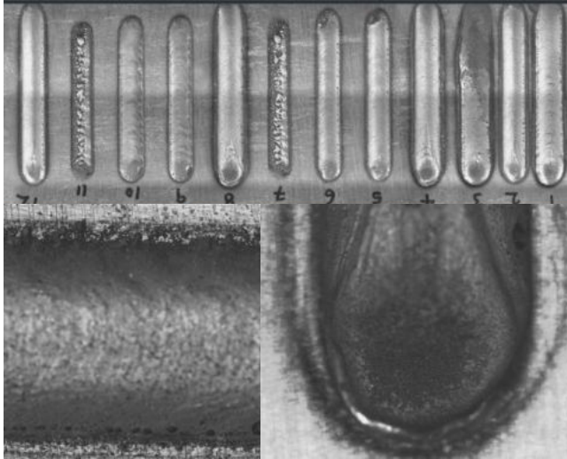
Laser-powder (LP) DED
