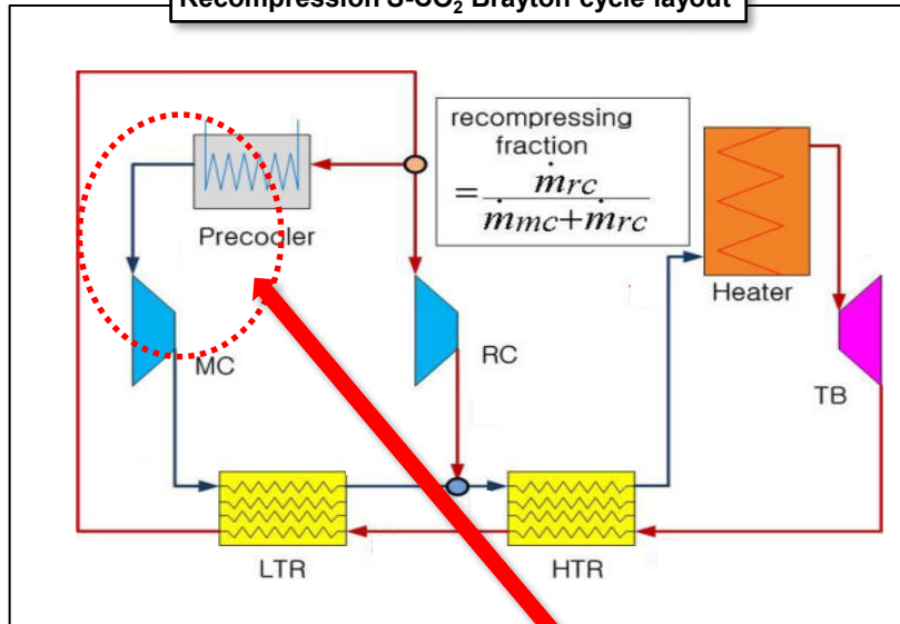
Recompression S-CO 2 Brayton cycle layout
