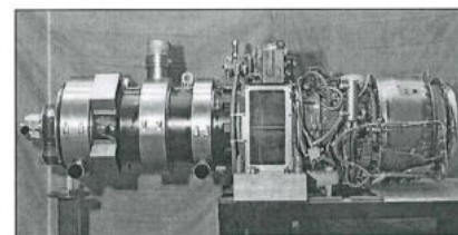
Figure 2: ALPS HS-Generator mounted with a Navy TF40b engine.
