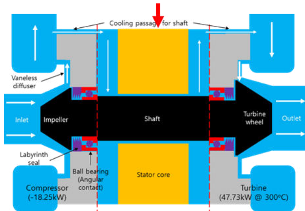
Fig. Schematic diagram of S-CO 2 TAC (40000 RPM, PR=1.29, \dot{m} =3 kg/s @ Design point)
