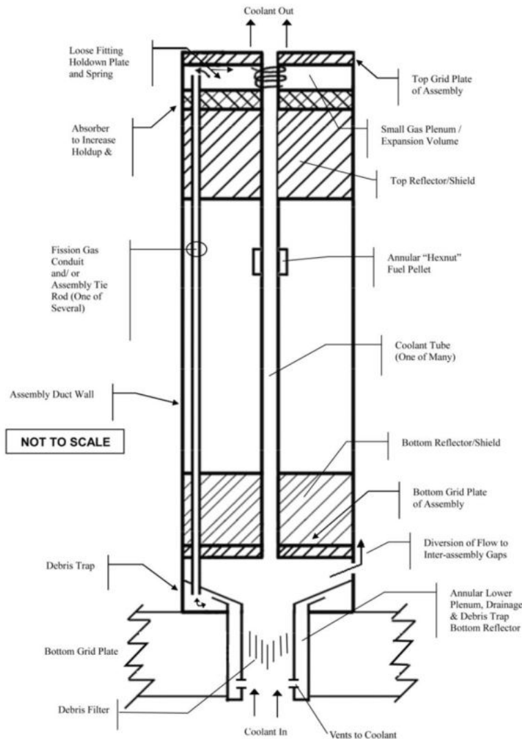
<Vented Fuel>
