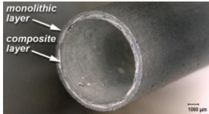
General Atomics SiGA ® SiC composite cladding tube
