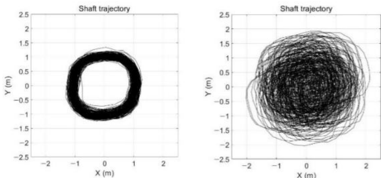
Fig. Shaft trajectory data, vacuum(left), S-CO 2 (right)
