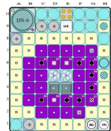
Typical core layouts with in-fuel irradiation rig in position
