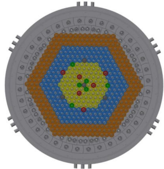
ALLEGRO RPV cross-section
