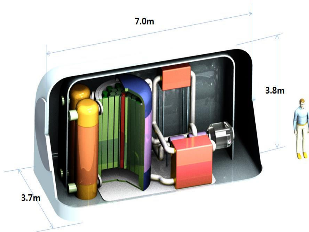
<Configuration of MMR>
