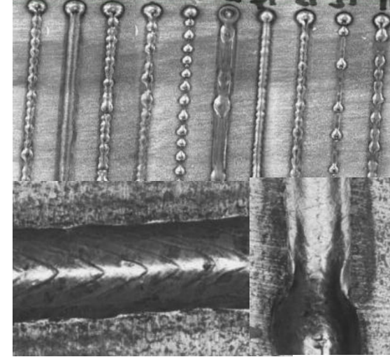
Arc-wire (AW) DED
