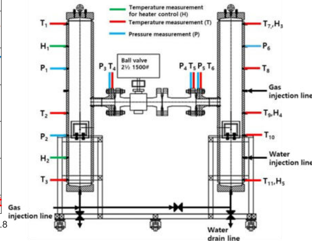
Fig. Schematic(Left) and photograph(Right) of facility
