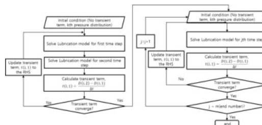
Fig. Lubrication analysis flow chart
