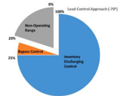
Best Control Scheme Change for Different Compressor Designs
