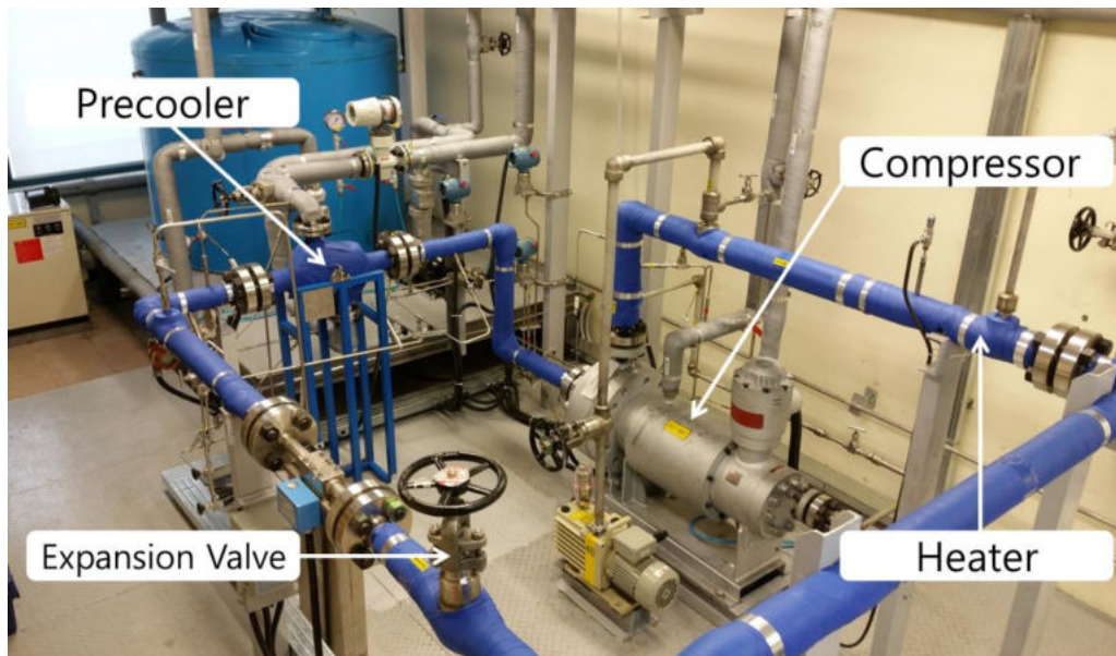
<SCO 2 PE facility modeling with modified GAMMA+ code>
