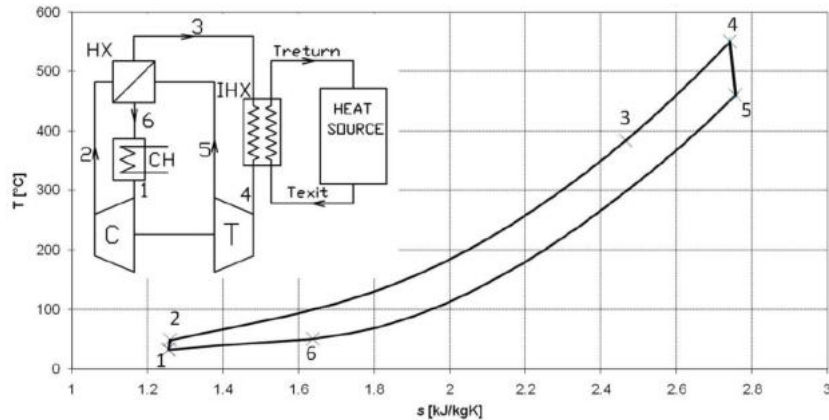
Simple Brayton Cycle Temperature - Entropy Diagram
