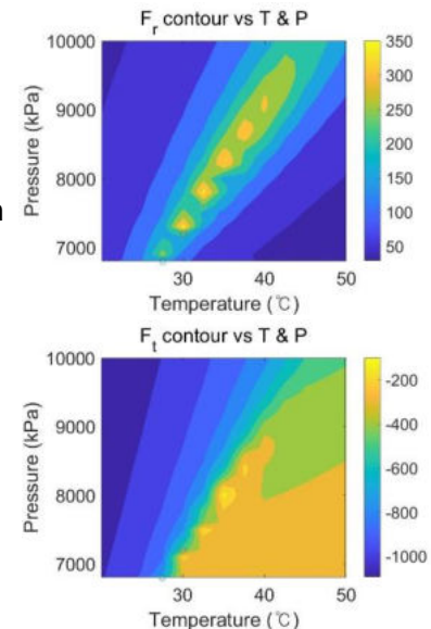
Fig. Lubrication force vs. CO 2 condition
